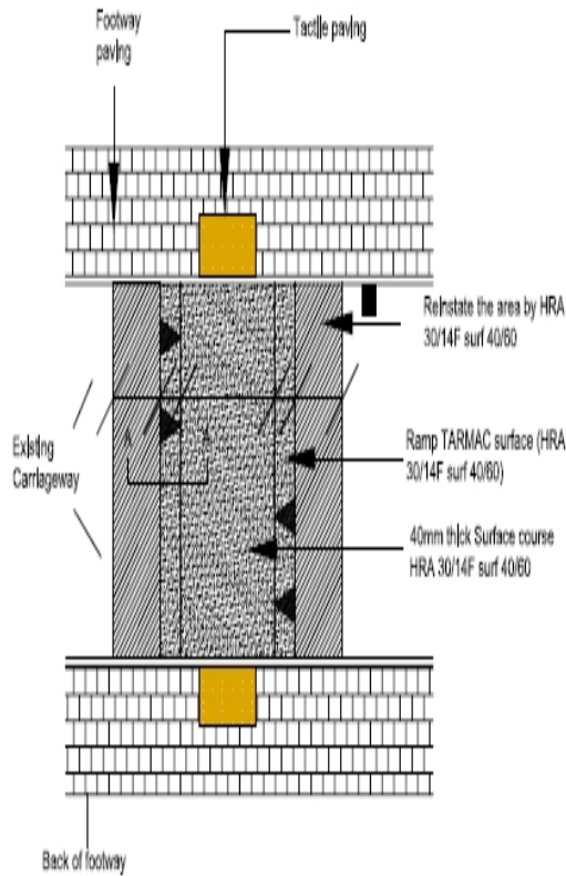
TYPICAL ASPHALT SPEED TABLE
